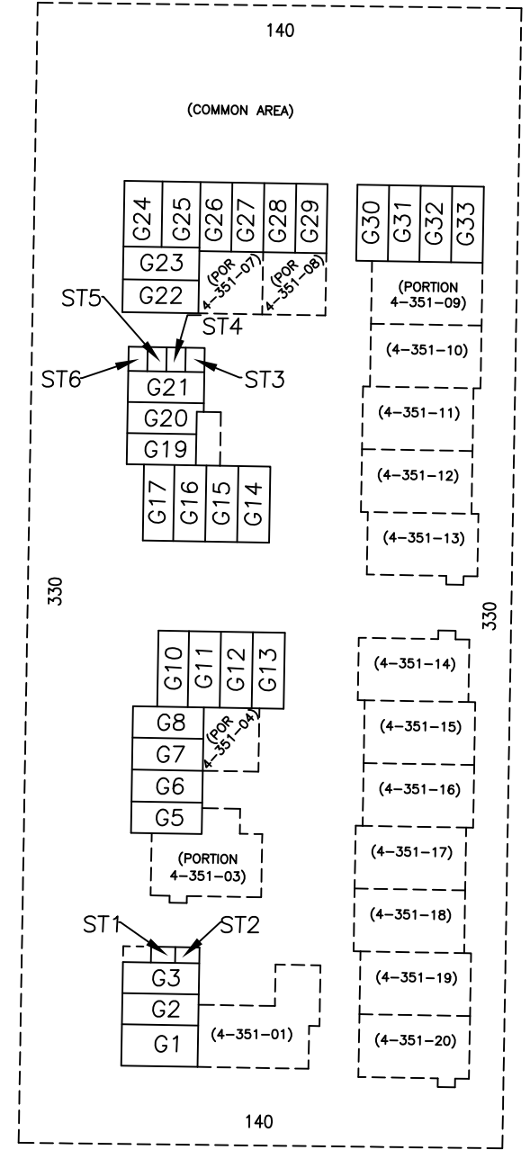
EXCLUSIVE EASEMENT PLAN FIRST FLOOR AREA OF TOWNHOMES, GARAGES, AND PRIVATE STORAGE UNITS.
